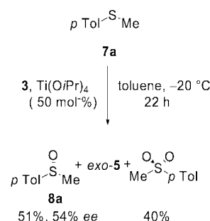
Scheme 4. Combined stereoconvergent oxidations of sulfide 7a . Molar ratios: 7a / 3 :1/2.
