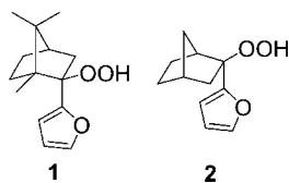
Figure 1. ( R )-camphor- and ( S )-norcamphor-based tertiary hydroperoxides.
