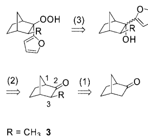
Scheme 1. Retrosynthetic approach to functionalized ( S )-norcamphor-based hydroperoxides.
